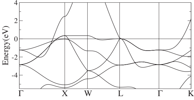
FIG. 6. The band structure of fcc Pd. The Fermi level is fixed at 0 eV.
