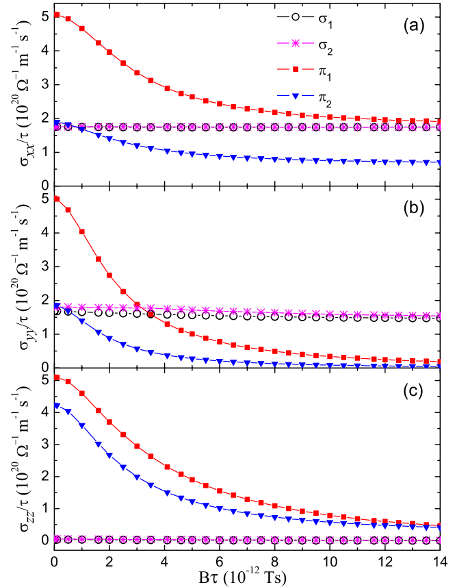
FIG. 5. (Color online) B\tau dependences of (a) \sigma_{xx}/\tau , (b) \sigma_{yy}/\tau , and (c) \sigma_{zz}/\tau of the four bands of MgB 2 . The magnetic field is applied along the x axis in the ab plane.
