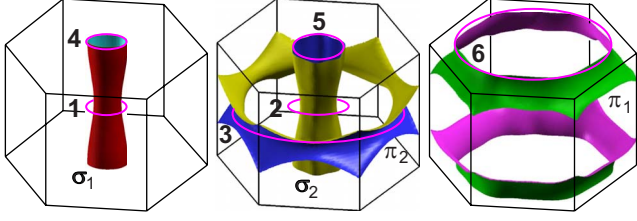
FIG. 1. (Color online) The calculated Fermi surface of \text{MgB}_2 and the extremal orbits labeled for the magnetic field along the c axis.
