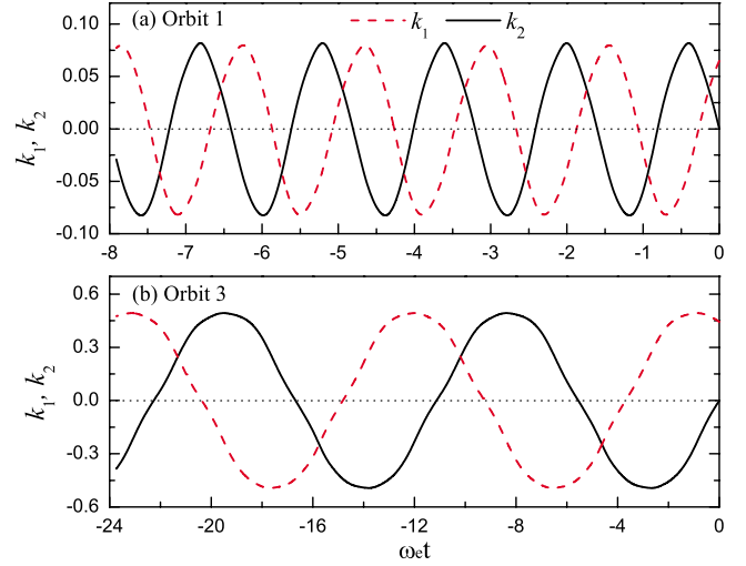
FIG. 3. (Color online) Historical track of the electron wave packet in reciprocal space. The initial positions are (a) \mathbf{k}(0.065, 0.0, 0.0) in orbit 1 and (b) \mathbf{k}(0.444, 0.0, 0.0) in orbit 3, respectively. \mathbf{k} points are expressed as \mathbf{k}(k_1, k_2, k_3) in the unit of reciprocal lattice vectors. There are 4000 points on each curve. k_3 is fixed in the \Gamma plane during the simulation. The abscissa \omega_e t is related to Bt as \omega_e t = \frac{e}{m_e} Bt where m_e is the mass of a free electron.
